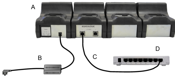
Figure 3 - Ethernet Connection
